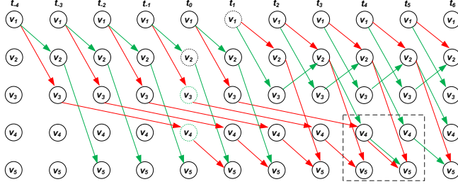
(c) A possible update sequence in the time-extended network resulting from two-phase update protocols . We assume the time difference between the first phase and the second phase is one time step. We can observe that the congestion happens at the link \langle v_4(t_4), v_5(t_5) \rangle .
