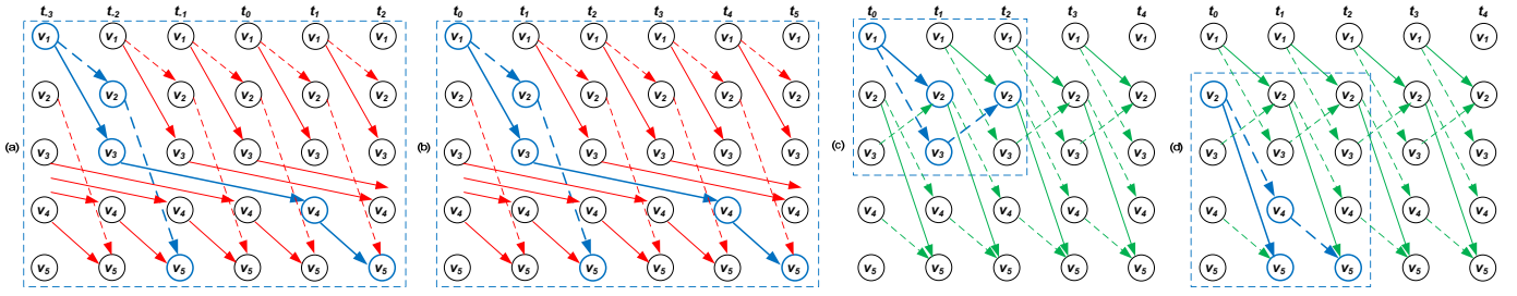
Fig. 5. Four update blocks (colored blue) (a) o_1^{f_r}(t_{-3}) , (b) o_1^{f_r}(t_0) , (c) o_1^{f_g}(t_0) and (d) o_2^{f_g}(t_0) in the time-extended network for red flow f_r and green flow f_g of Fig. 1(b).
