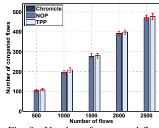
Fig. 9. Number of congested flows
