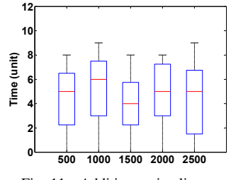
Fig. 11. Additive optimality gap
