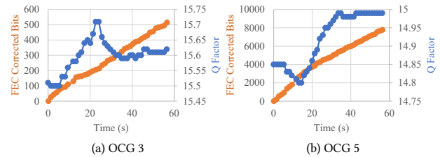
Figure 6: QoT measurements for witness waves while adding/dropping OCG1. During the add/drop, Q factor for the witness waves is relatively constant—varying by +/- 0.1. Errors accumulate at a linear rate as expected in a live transport network; 100% are corrected with FEC while running traffic over OCGs 3 and 5.
