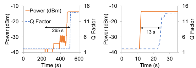
(a) Automatic mode: add-time is 4 min (b) Manual mode: add-time is 13 s—over and 25 s. Hence, today's WANs are not 19× faster than automatic mode (Figure 1a).
